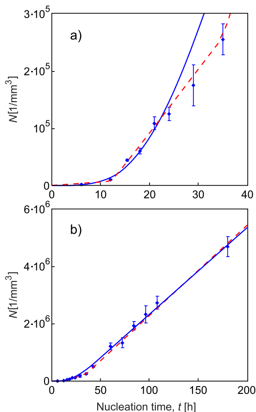
FIG. 5. Crystal number density vs nucleation time at 713 K. Rhombuses are the experimental data. The solid blue line was plotted by Eq. (9) with \zeta(t) approximated by the Kohlrausch stretched exponent equation [Eq. (8)]. The dashed red line corresponds to the stepwise evolution of the structural order parameter that allows the best description of the experimental data. Indexes correspond to different nucleation times considered in this analysis: short (a) and average (b) observations.
